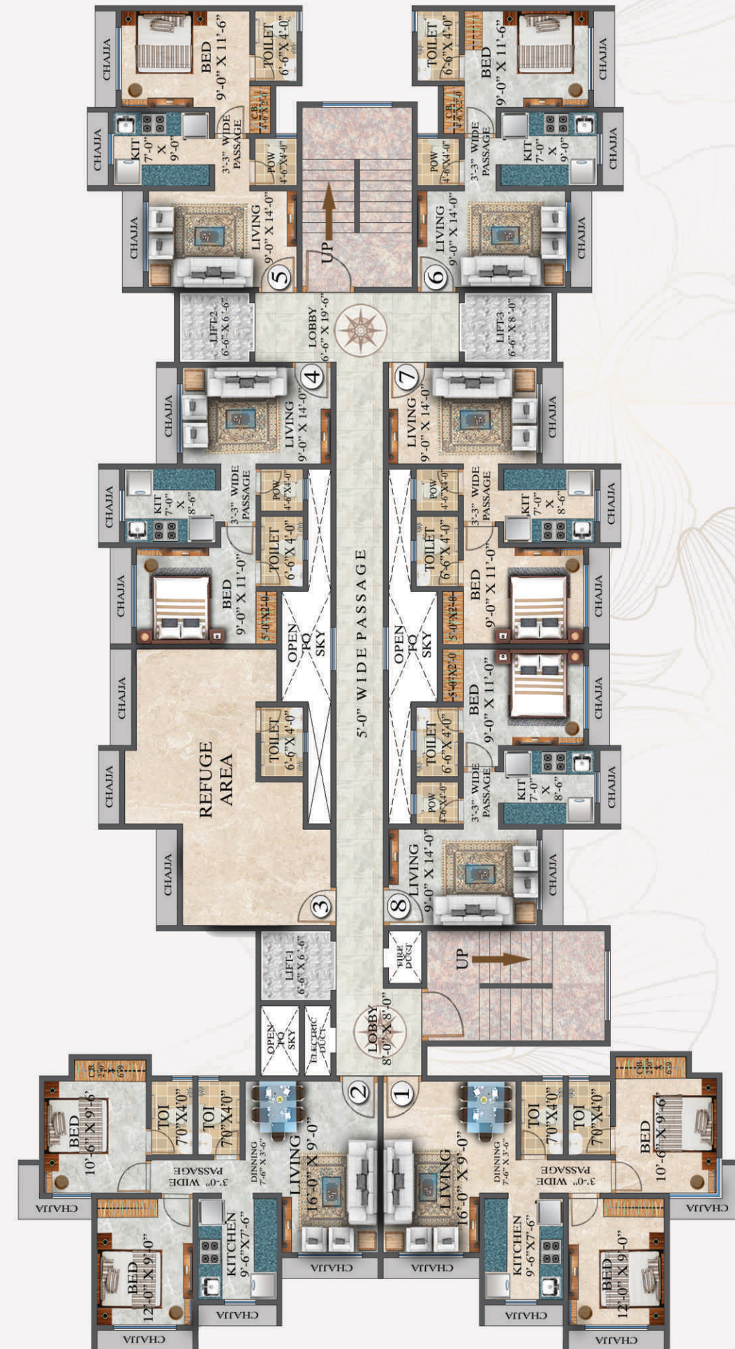
REFUGE FLOOR PLAN 13TH & 18TH FLOOR
