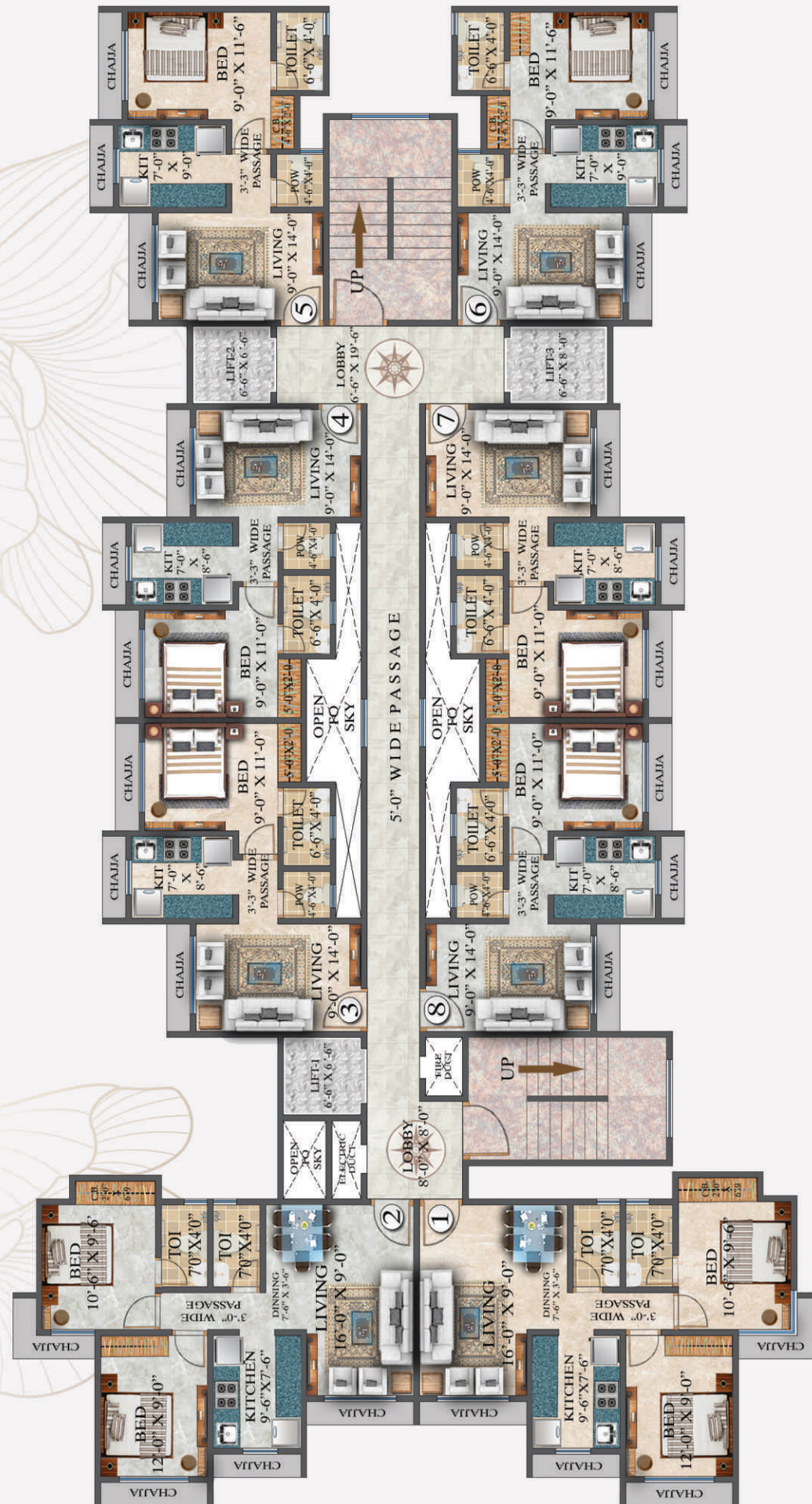
TYPICAL FLOOR PLAN 3RD TO 7TH, 9TH TO 12TH, 14TH TO 17TH, 19TH TO 21ST FLOOR
